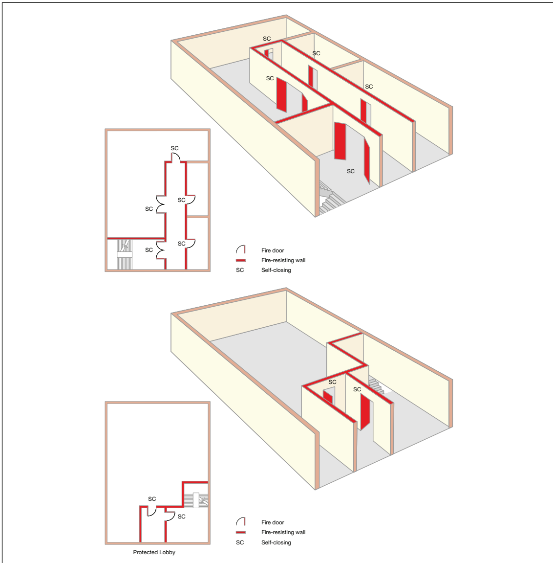
Figure 35: Examples of a stairway with protected lobby/corridor approach
