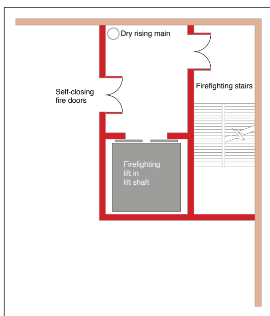
Figure 21: Firefighting shaft
