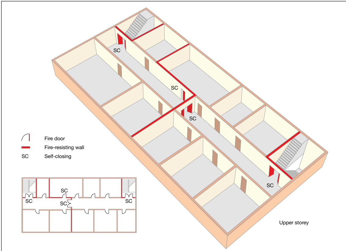
Figure 34: Subdivision of corridor between two stairways or exits
