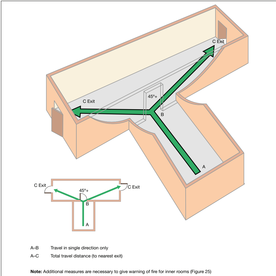
Figure 29: Measuring travel distance from initial dead end (inner room)
