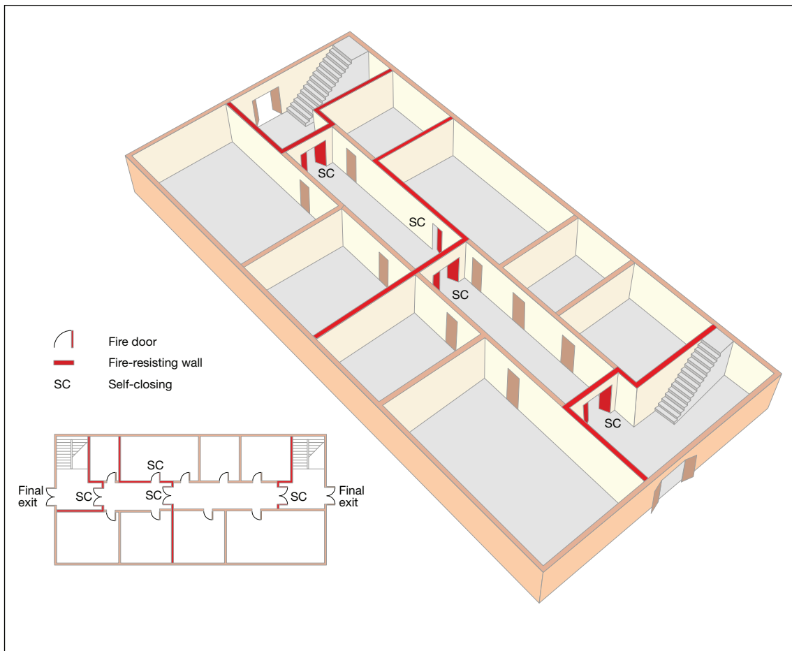
Figure 38: Separation of protected stairways
