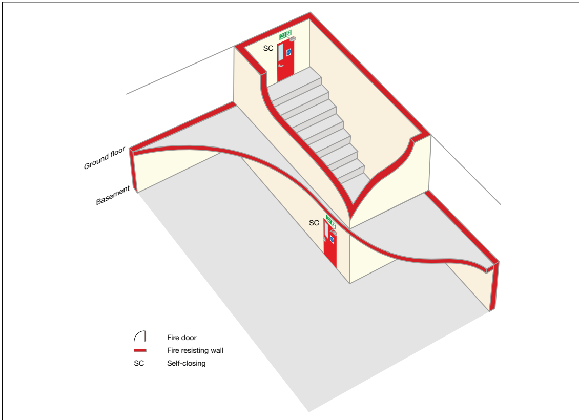
Figure 33: Basement protection
