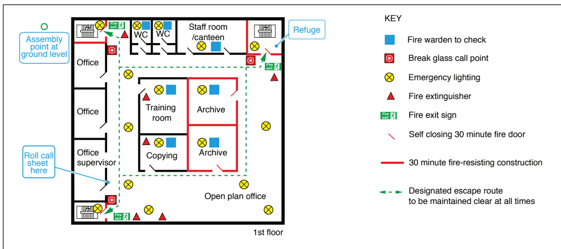
Figure 12: Example of a line drawing showing general fire safety precautions
