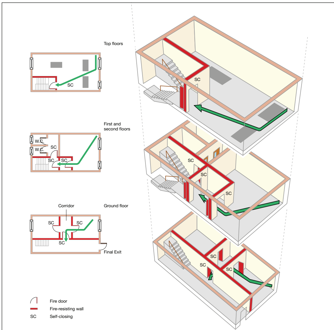
Figure 50: Shop premises, ground and up to three upper storeys - protected lobbies/corridors
