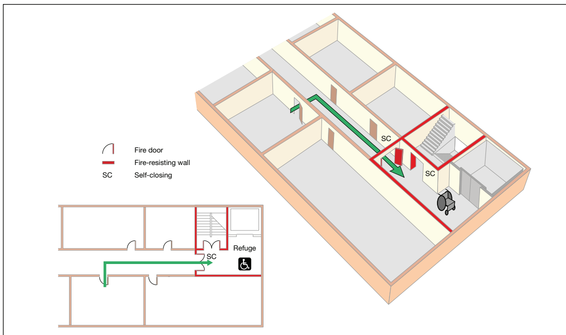
Figure 23: An example of a refuge
