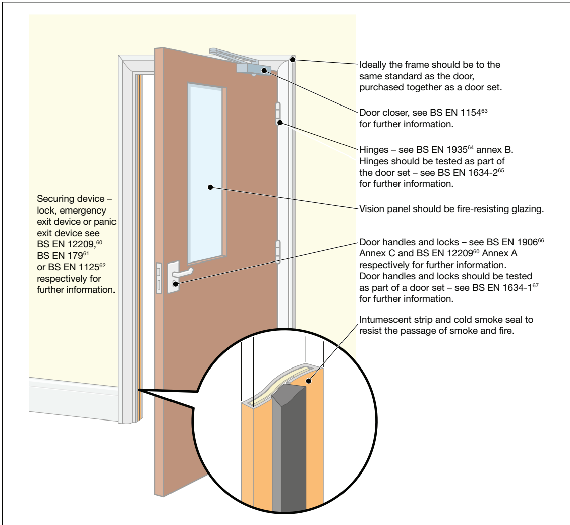
Figure 63: A fire-resisting and smoke-stopping door
