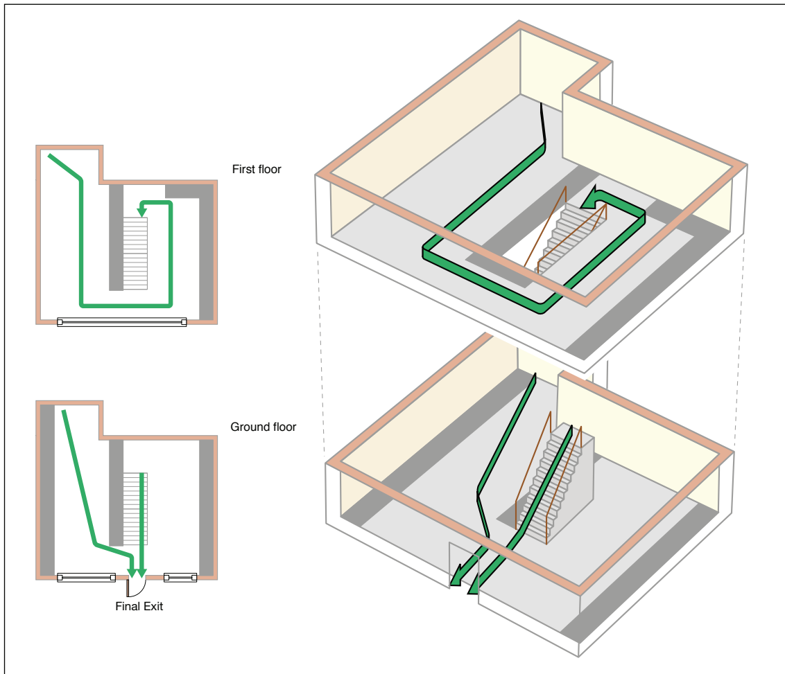
Figure 45: Two-storey premises
