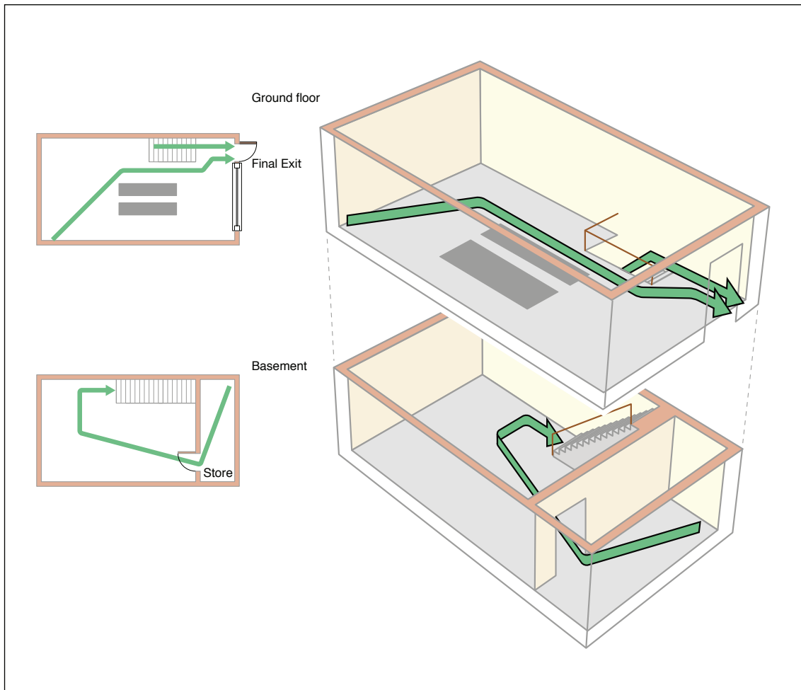
Figure 46: Two-storey premises, including basement
