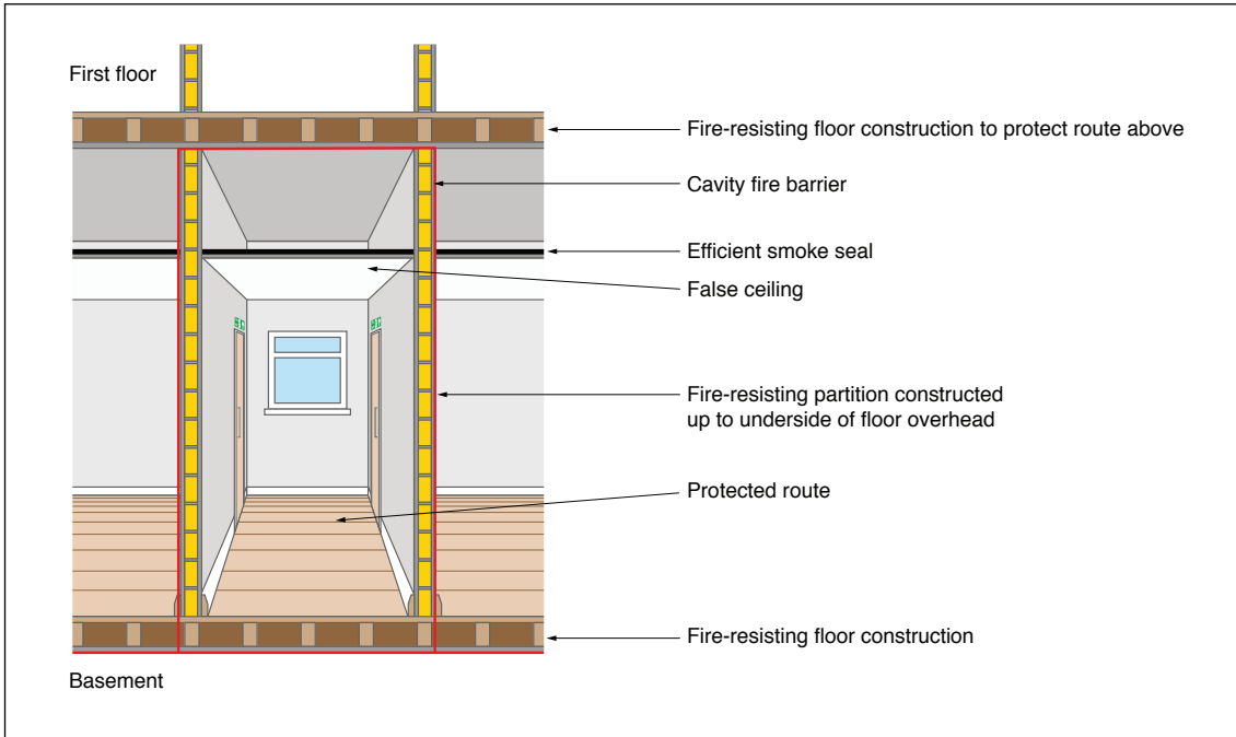
Figure 62: Fire-resisting construction
