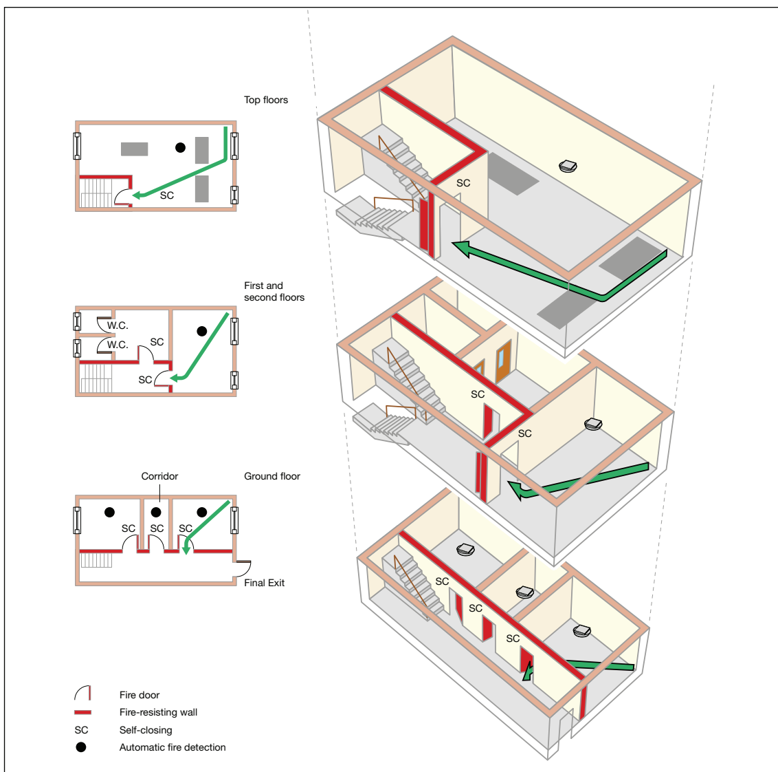
Figure 51: Shop premises, ground and up to three upper storeys - automatic fire detection
