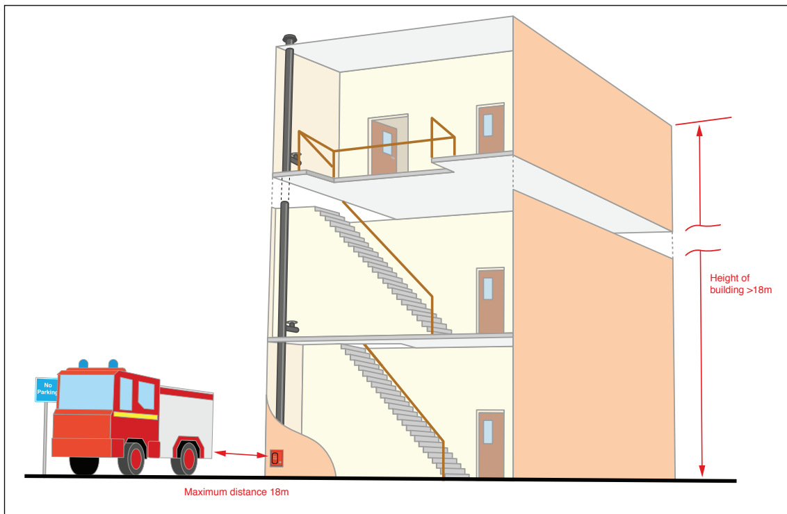
Figure 22: Rising main
