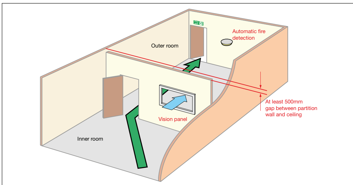
Figure 25: Inner rooms
