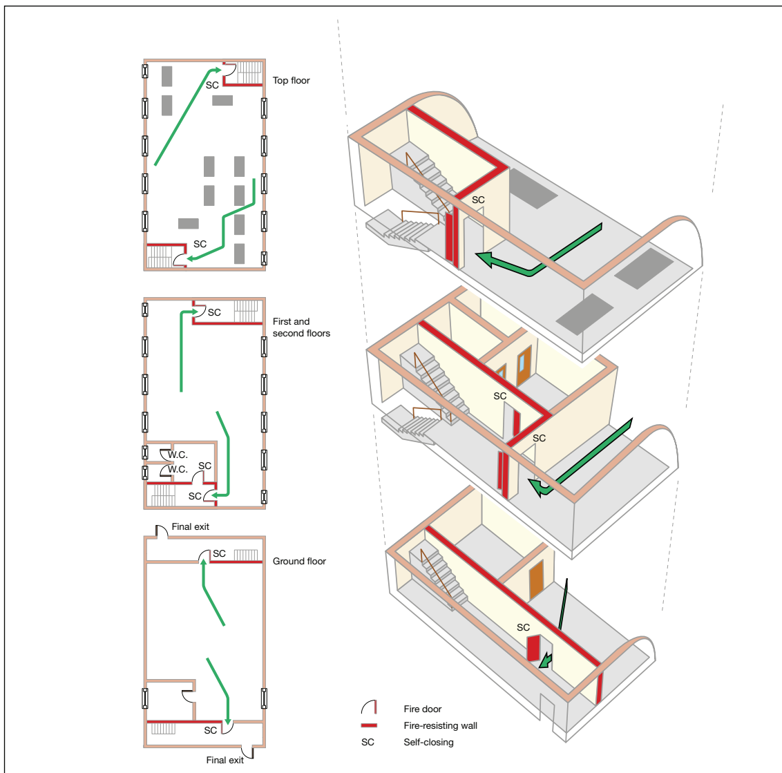
Figure 52: Example of a multi-storey building
