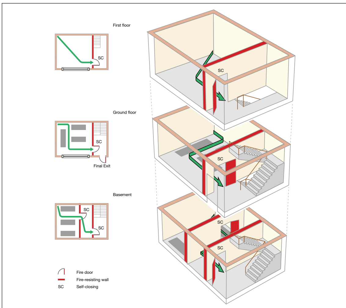
Figure 48: Larger three-storey premises, including basement
